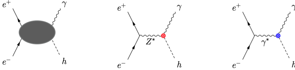
Figure 3: Diagrams arising from each of the three terms of Equation 1, respectively.
