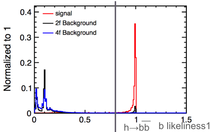
Figure 5: The distribution of b -likeness for signal and background events with unit normalization
